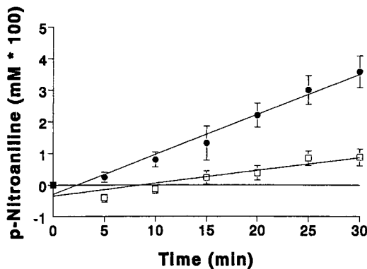
Fig. 4. Dipeptidyl peptidase IV (DP IV) activity as measured by temporal production of p -nitroaniline from Gly-Pro- p -nitroanilide in plasma from normal HCs (●; n = 6 ) and patients with inflammatory bowel disease (IBD; □; n = 5 with CD and n = 1 with UC). P < 0.05 for IBD vs. normal HCs.
